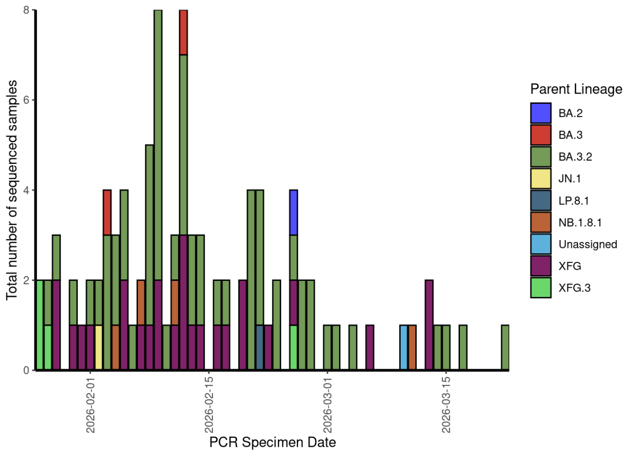
Figure 2.1: Sequenced COVID-19 cases in Northern Ireland, by parent lineage and day, for the last 8 weeks of sequencing data
