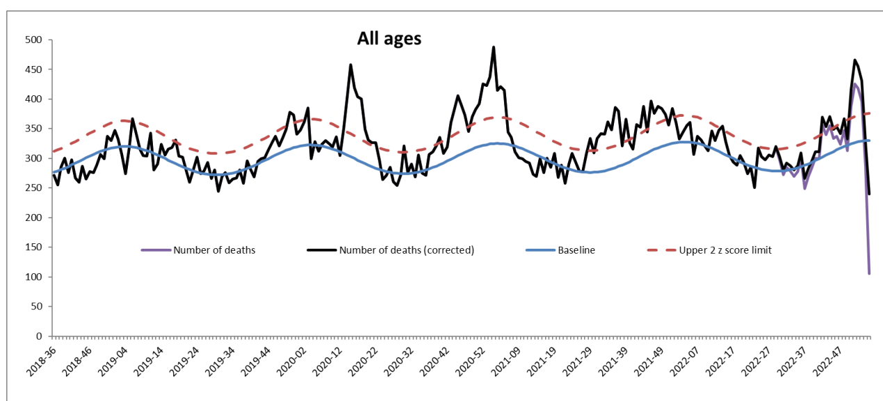
Figure 6. Weekly observed and expected number of all-cause deaths in all ages, week 36, 2018 – week 3, 2023
