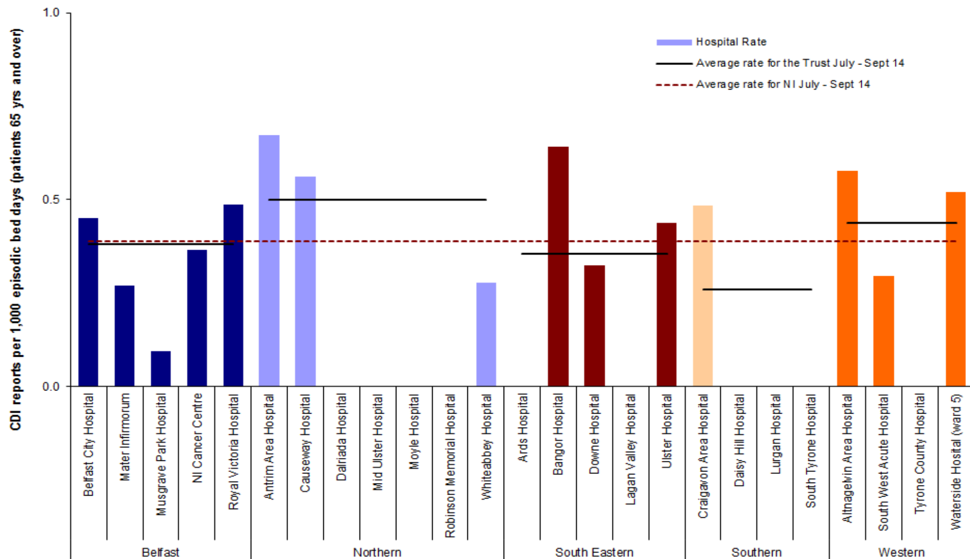
Figure 5: Rates of C. difficile in quarter three 2014 among inpatients aged 65 years and over, by hospital, including the quarterly HSCT rates and an average rate for Northern Ireland (see appendix A, Table 3)
