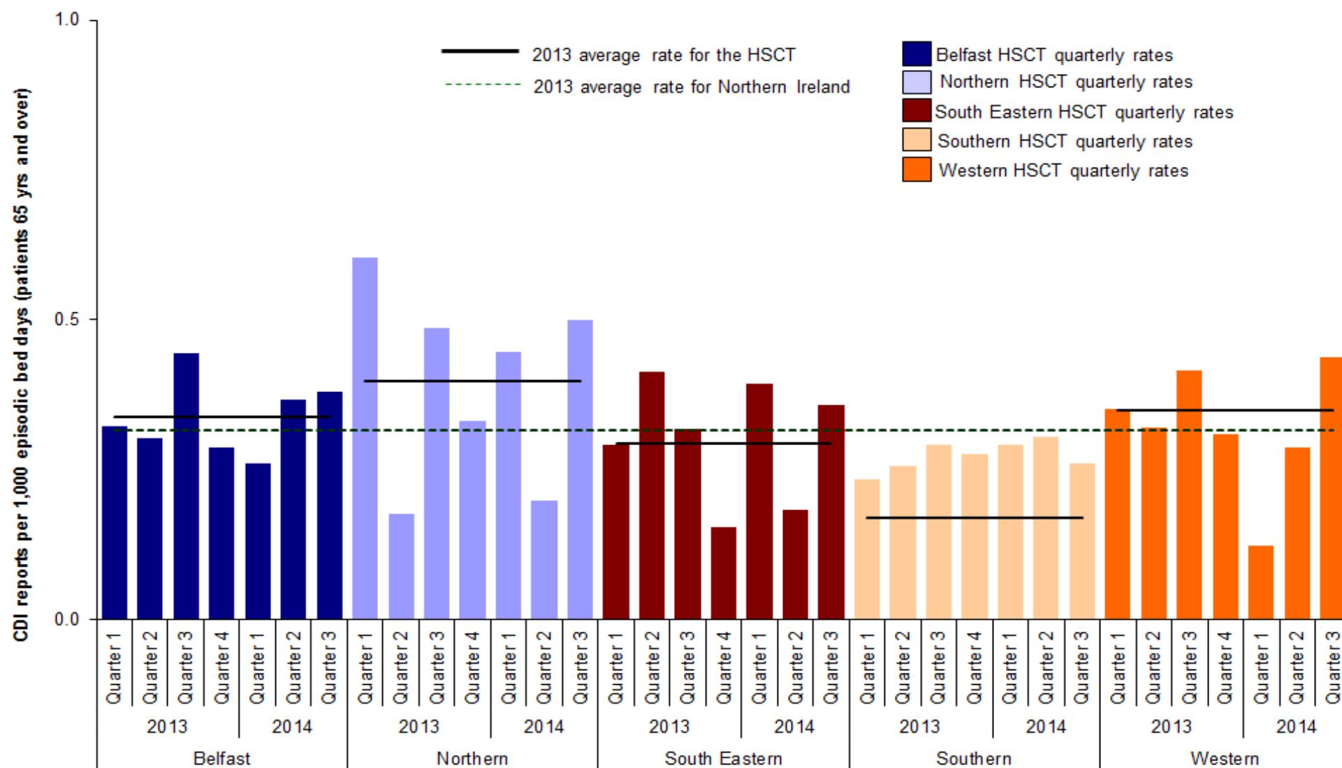
Figure 4: Quarterly rates of C. difficile among inpatients aged 65 years and over, by HSCT, 1 January 2013 - 30 September 2014, compared with annual Northern Ireland and HSCT rates for 2013
