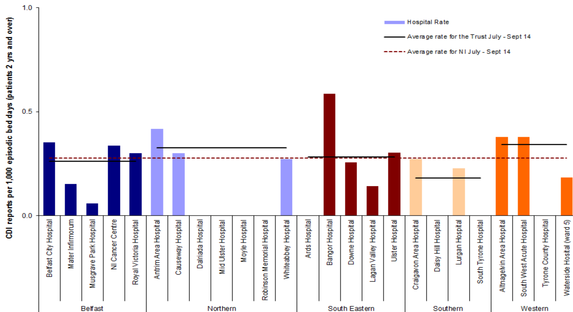
Figure 6: Rates of C. difficile in quarter three 2014 among inpatients aged two years and over, by hospital, including the quarterly HSCT rates and an average rate for Northern Ireland (see appendix A, Table 4)
